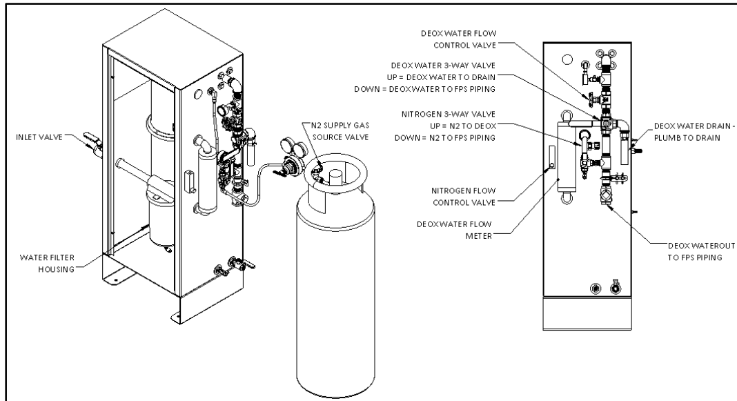
Figure 9: Operation Procedure 2
