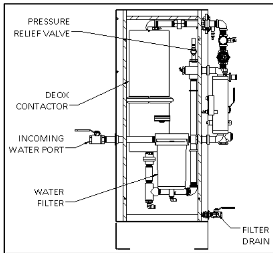
Figure 12: Water Filter
